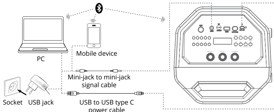
Fig. 3. Connection diagram
