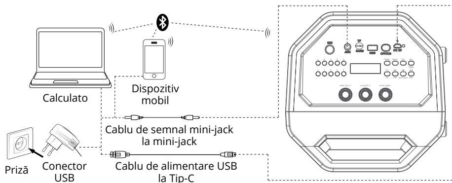
Fig. 3. Connection diagram
