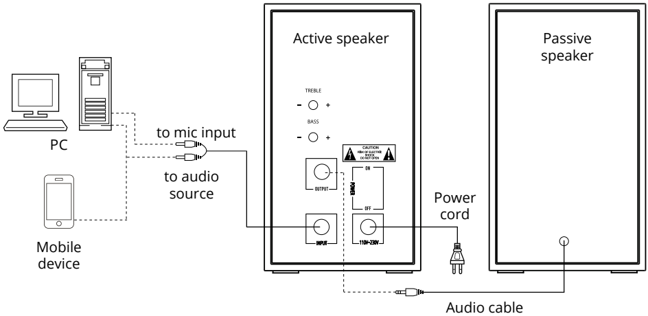
Fig. 2. Connection diagram
