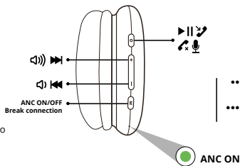
Fig. 3. Button functions
