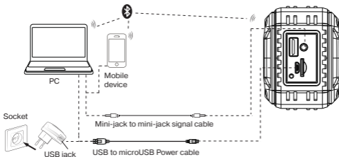
Fig. 2. Connection diagram
