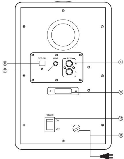
Fig. 3. Active speaker rear panel
